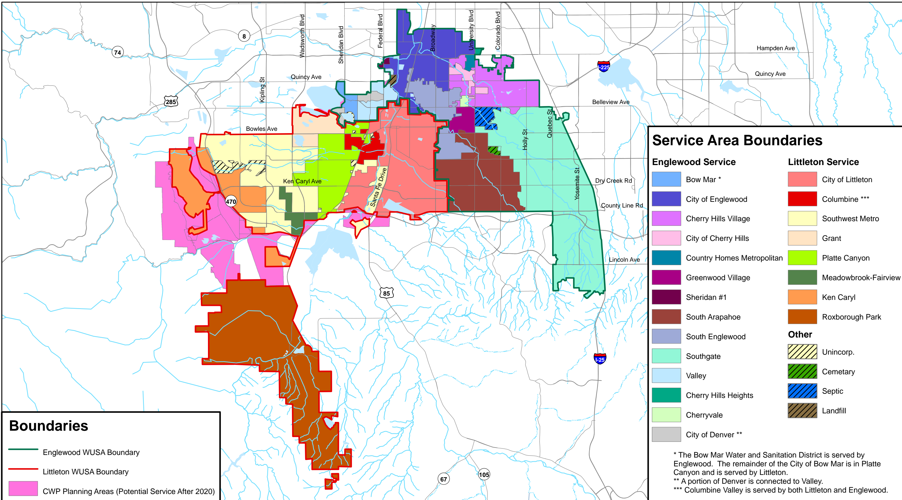
Figure 4-1. L/E WWTP WUSA and CWP Planning Area
